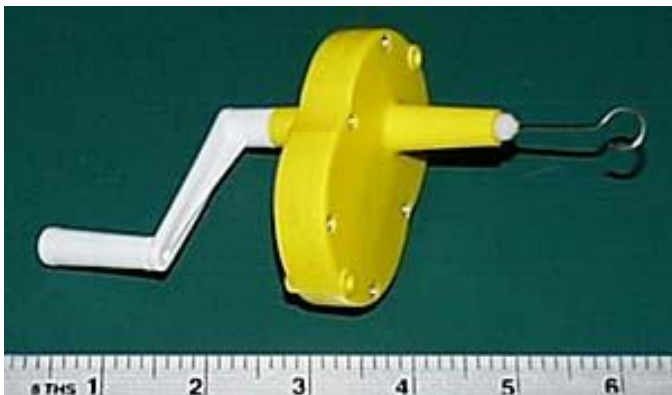
Here's a typical rubber motor winder. This one has a gear ratio of 10:1. One turn of the handle gives ten turns of the winding hook, speeding the winding process and enabling stretch winding of long motors.
